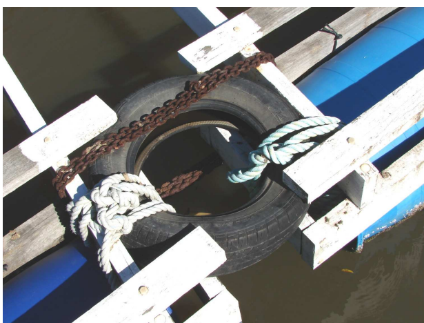
Figure 11. A small car tyre fitted between consecutive rafts in a raft complex as a shock absorbing and spacing device. Note the use of a secondary safety chain. In practice tyres should be attached at four diagonal points to the raft to minimise side slip.
