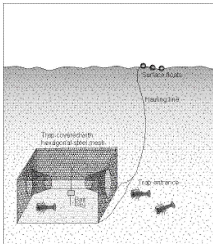
Figure B1.5 Lobster trap commonly used in the offshore area of the Lobster Fishery.
