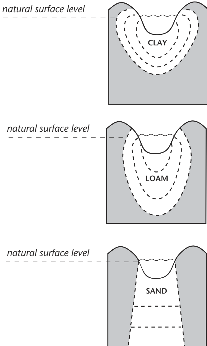
Figure 6. Wetting patterns within furrows
