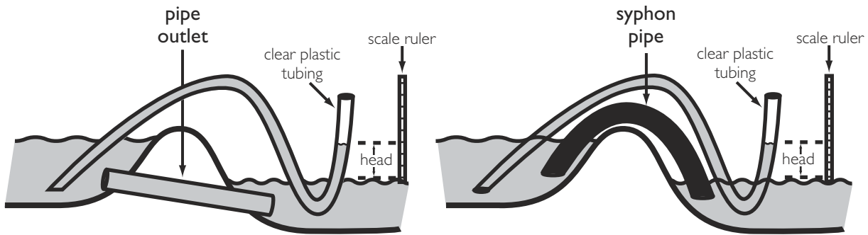
Figure 4. Measuring head over a field or bay
