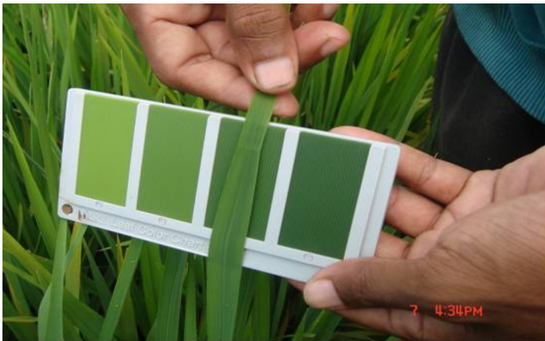
Figure 1. Using Leaf Colour Chart for measuring leaf colour in determining N fertilization in rice crop.
