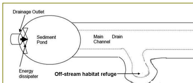
Sediment ponds and energy dissipaters slow down stormwater entering drains. Illustration: Richmond Valley Council
