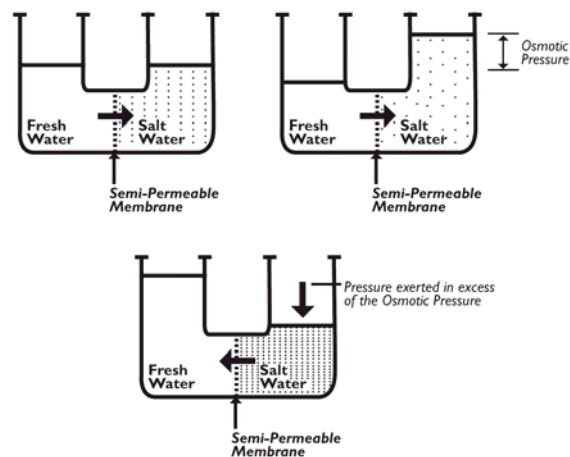
Figure 1. How a reverse osmosis unit works.
