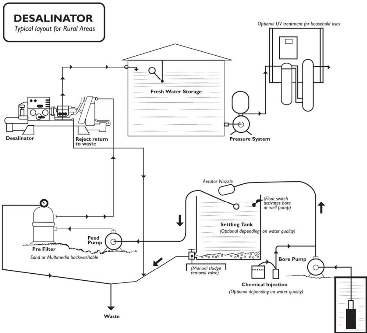
Figure 2. A typical desalination layout for rural areas
