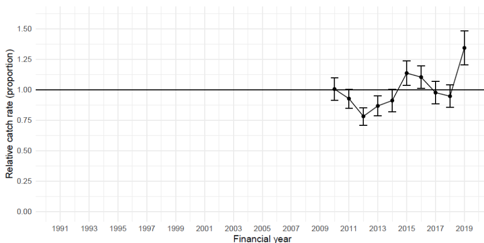
Figure 10 Annual relative standardised catch rates of Stout Whiting from the NSW Ocean Trawl Fishery (in kg per hour trawled scaled to the overall mean catch rate=1). Error bars indicate 95% confidence intervals. Reproduced from Wortmann and Hall (2021).
