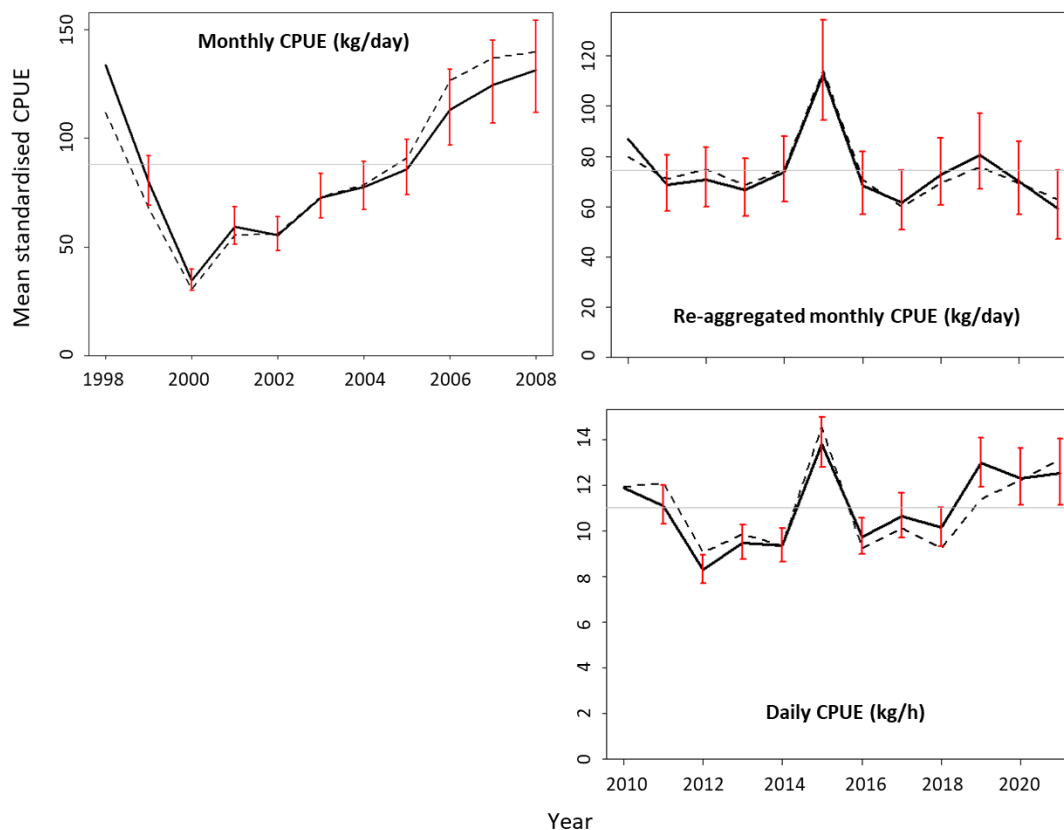
Figure 5 Mean standardised catch rates (catch-per-unit-effort, CPUE) of Stout Whiting for the ocean prawn trawl sector of the NSW Ocean Trawl Fishery, estimated from monthly records (1998–2009) and re-aggregated daily records (2010–2021) in kg per days fished and from daily fishing event records (2010–2021) in kg per hours trawled. The dashed and solid lines indicate the nominal and standardised mean CPUE ( \pm 95% confidence intervals), respectively; and the grey horizontal line indicates the long-term averages for each series.
