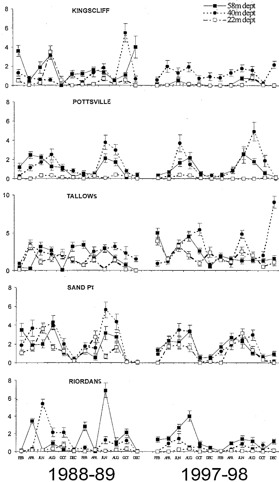
Figure 9. Fluctuations in the mean catch rate ( \pm SE) of legal-sized spanner crabs during both repeats of the survey at each location and depth ( n = 15 ).
