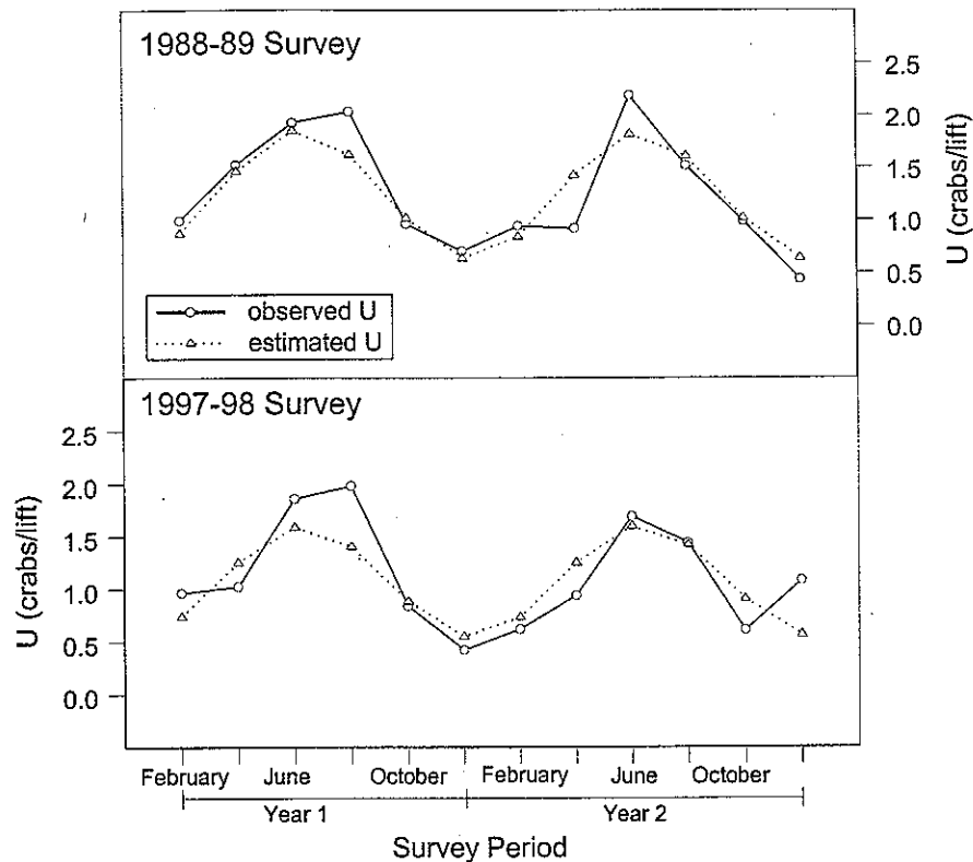
Figure 4. Comparison of the observed and estimated catch rates ( U_{obs} and U_{est} , measured in crabs/lift) for the two NSW spanner crabs surveys. Surveys were completed every two months (February, March, June, August, October and December) in 1988, 1989, 1997 and 1998.
