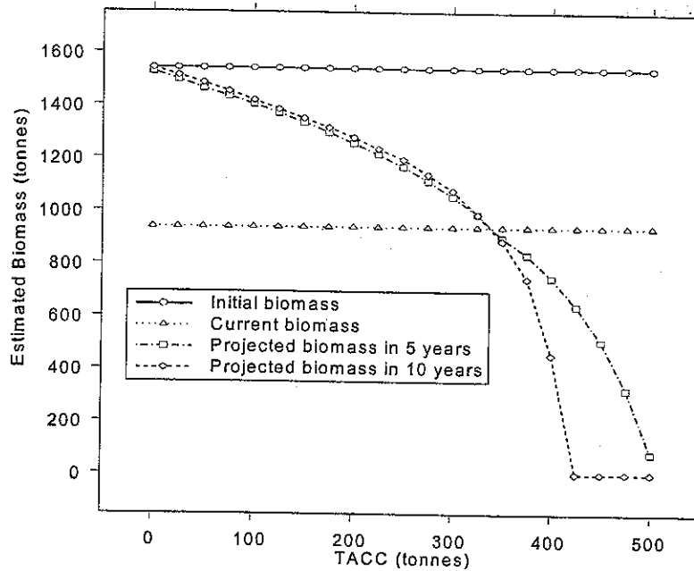
Figure 14. Plot of the median values of the biomass estimates for various total allowable commercial catches (TACC). The initial and current biomass estimates are independent of future TACC (as expected). There are rapid decreases in the projected biomass estimates once the TACC exceeds 350 tonnes.
