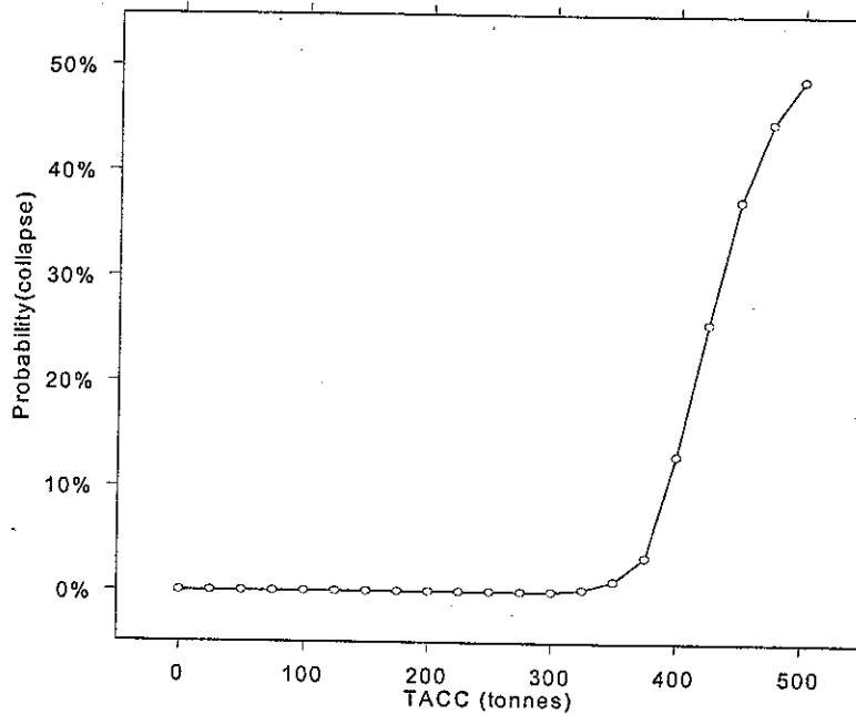
Figure 15. Plot illustrating the probability of collapse in the exploitable biomass as a function of TACC. Note that the spawning biomass is essentially not vulnerable in this fishery and there is no suggestion that the spawning stock will collapse. Risks to the exploitable stock become evident at a harvest rate of around 380 tonnes/year.
