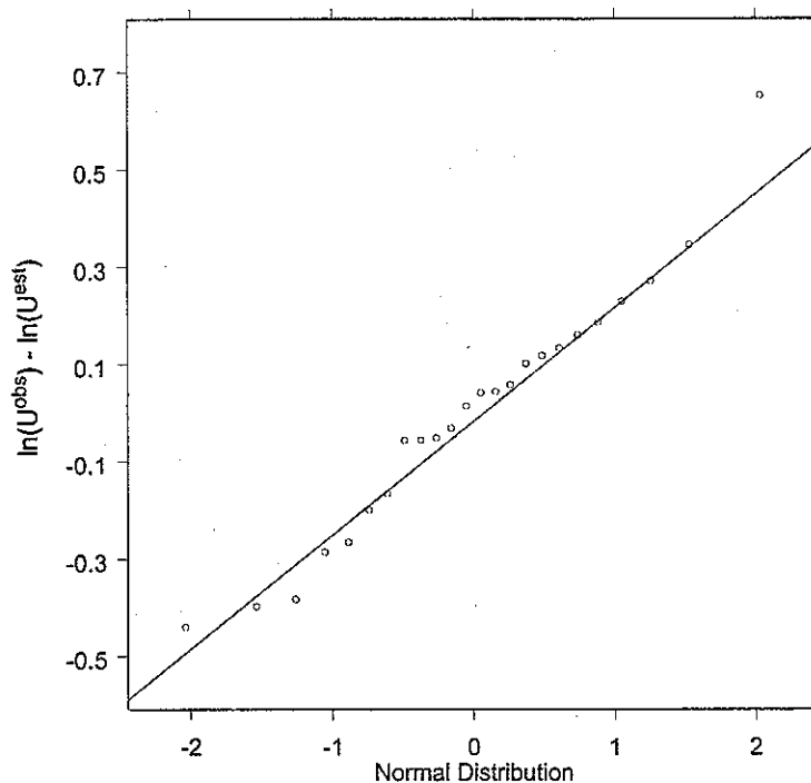
Figure 11. Quantile-quantile plot of the estimation errors (differences between the log of observed and log of estimated catch rates) from the model fit. The assumption that the error structure of the model is lognormal is supported by this figure.
