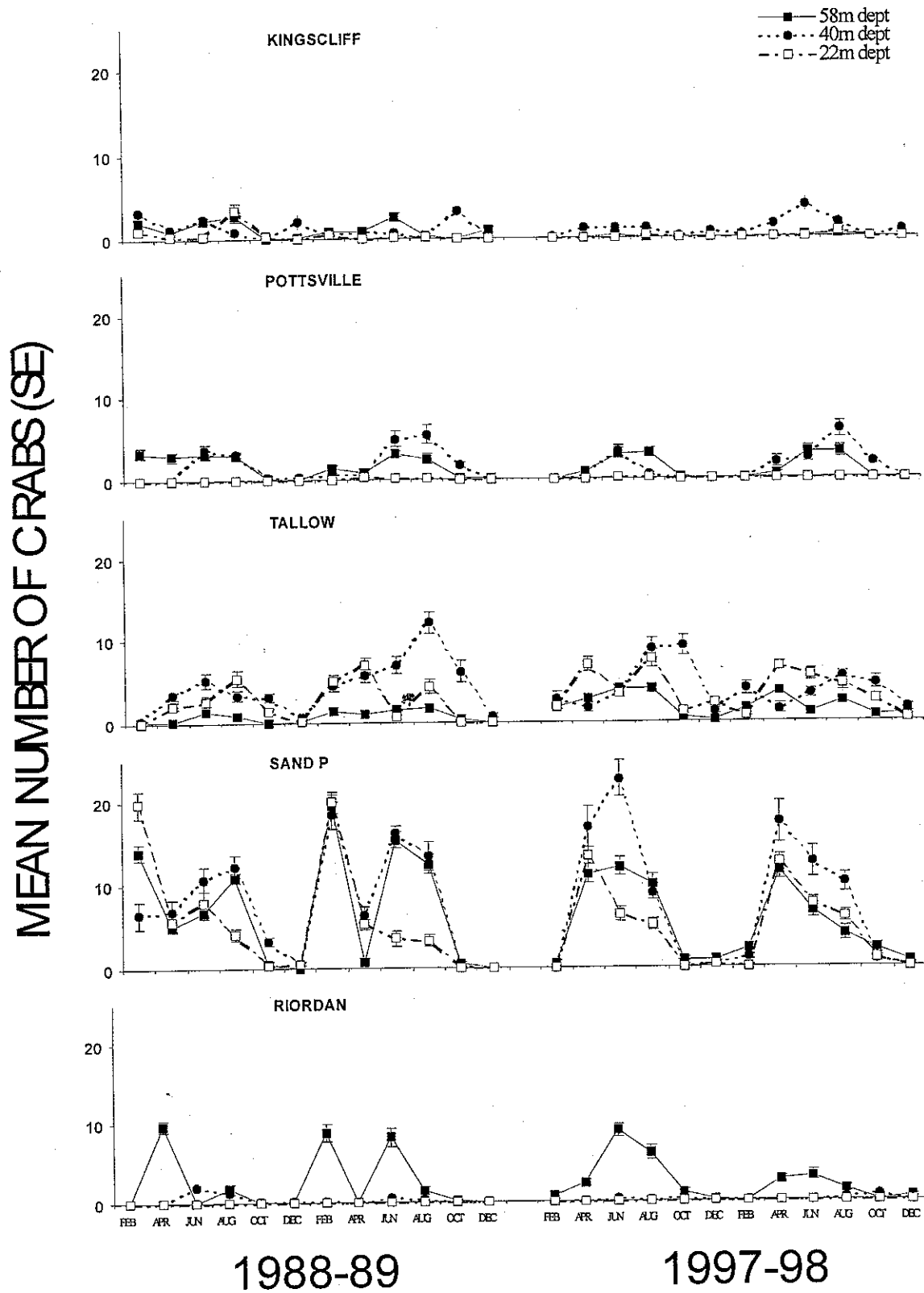
Figure 8. Fluctuations in the mean catch rate ( \pm SE) of female spanner crabs during both repeats of the survey at each location and depth ( n = 15 ).
