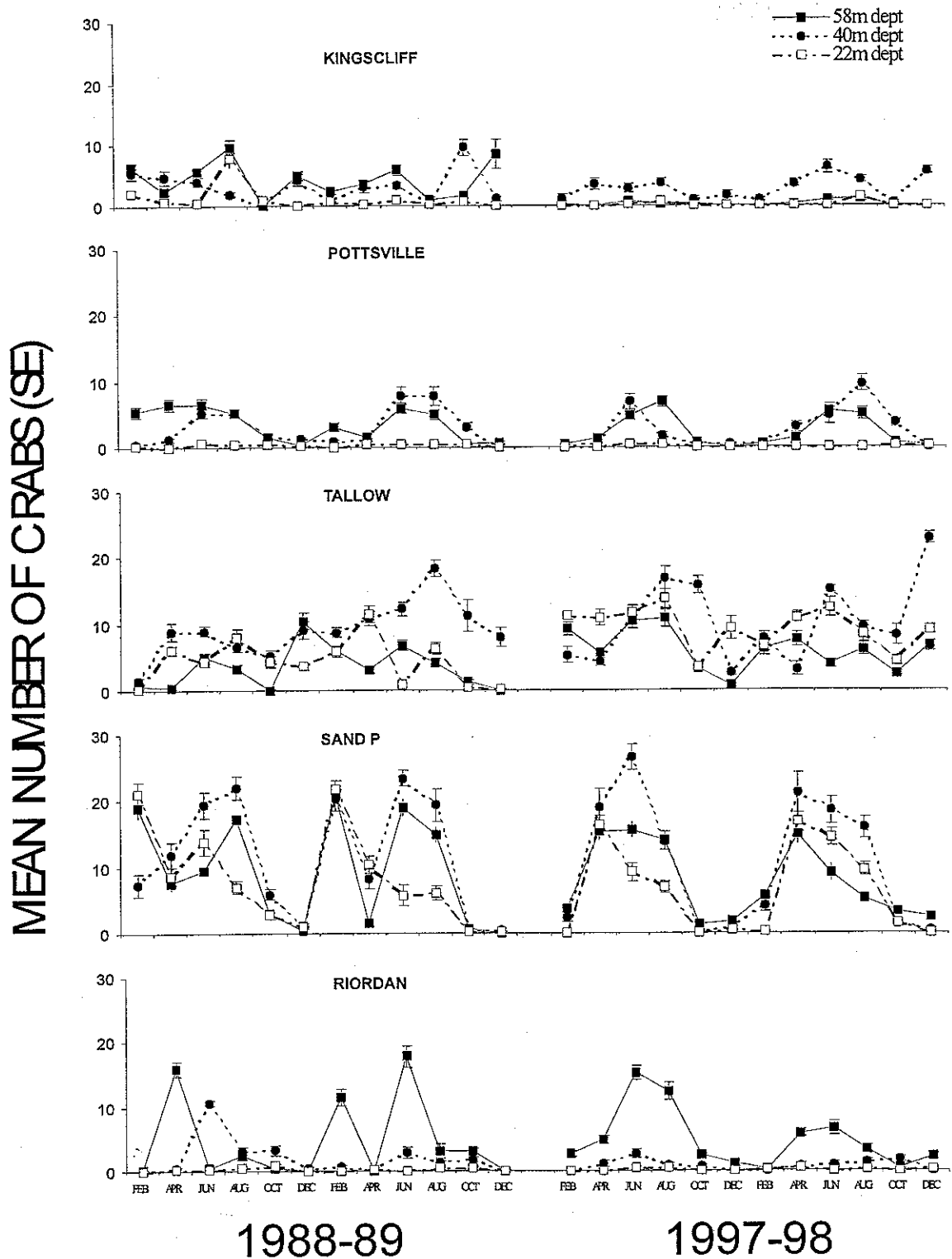
Figure 6. Fluctuations in the mean catch rate ( \pm SE) of spanner crabs during both repeats of the survey at each location and depth ( n = 15 ).
