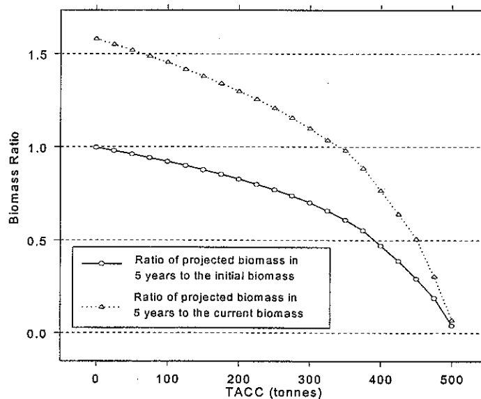
Figure 13. Plot of the median values of the ratios of biomass estimates for various total allowable commercial catches (TACC). The lower line indicates how the ratio of the biomass in 5 years time to the initial biomass changes over a range of harvest rates. The upper line gives that same ratio with respect to current (December 1998 biomass). A TACC of about 340 tonnes would maintain the current exploitable biomass with only 50% confidence.
