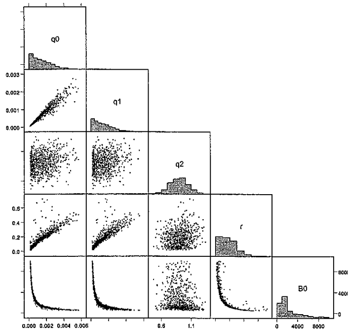
Figure 12. Scatterplot matrix illustrating parameter correlation and frequency distributions of the estimated parameters from the re-sampled datasets (after filtering). Subplots on the diagonal are frequency histograms of the annotated row or column variable. Off-diagonal subplots are scatterplots of the row variable versus column variable. Axis tick-marks indicate the scales of the annotated column or row variable. Strong inverse correlations between (q_0, B_0) , (q_1, B_0) and (r, B_0) are evident.
