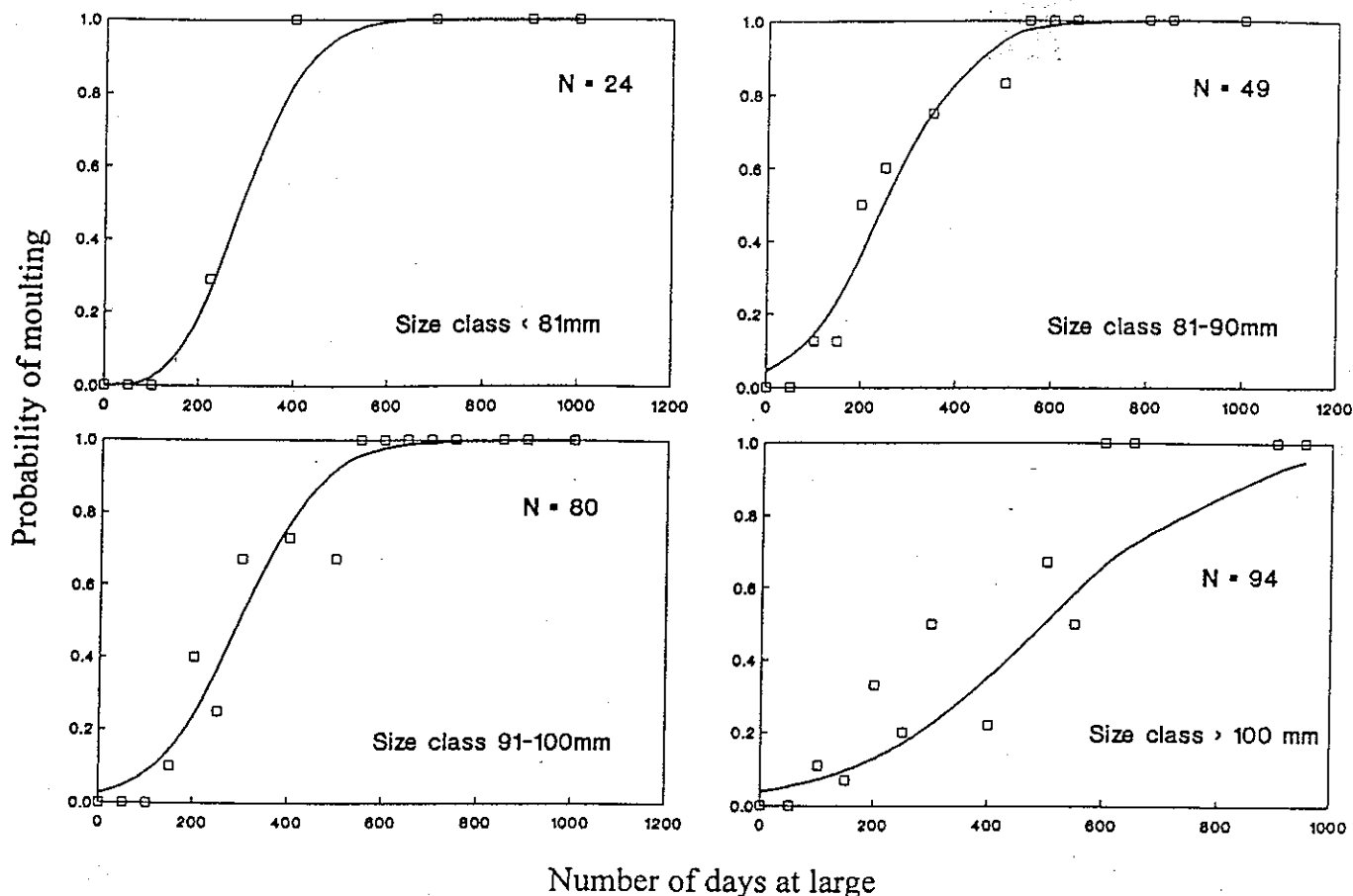
Fig. 3. Probability of moulting for male spanner crabs of different size classes in relation to the number of days at large: \square , observed value; curve, predicted value.
