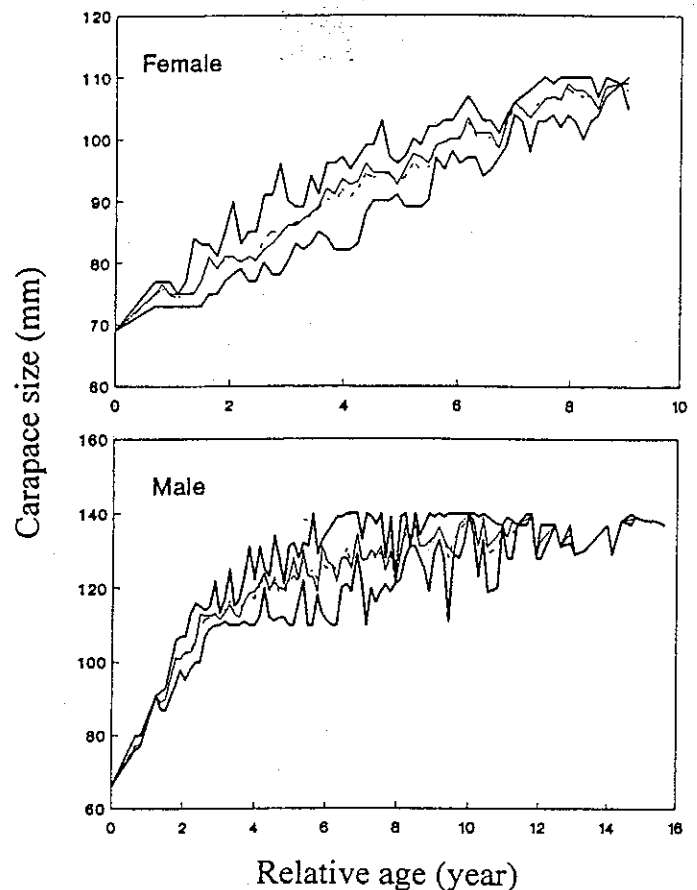
Fig. 7. Mean (dashed line), median (central thin line), and lower and upper 5th percentiles (outer thick lines) of carapace size at (relative) age resulting from 100 simulation runs using the probabilistic stepwise growth simulation approach.
