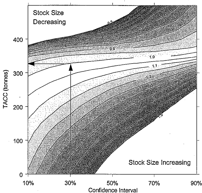
Figure 16. A contour plot of the ratio of the projected biomass in 5 years to the estimate of the current biomass as a function of TACC and projection uncertainty. The contour marked 1.00 indicates the TACC and confidence relationship where no change in the exploitable biomass will occur over the next 5 years. The lower right area indicates the region where the exploitable stock is likely to recover and the upper left where the exploitable biomass will decline. If you require 70% confidence that the exploitable stock size will remain the same over five years, move vertically from the 30% tick-mark on the horizontal axis to the contour marked 1.00 and then left to find the appropriate TACC (about 330 tonnes). Greater confidence in the outcome would require harvesting a lesser biomass of crabs.
