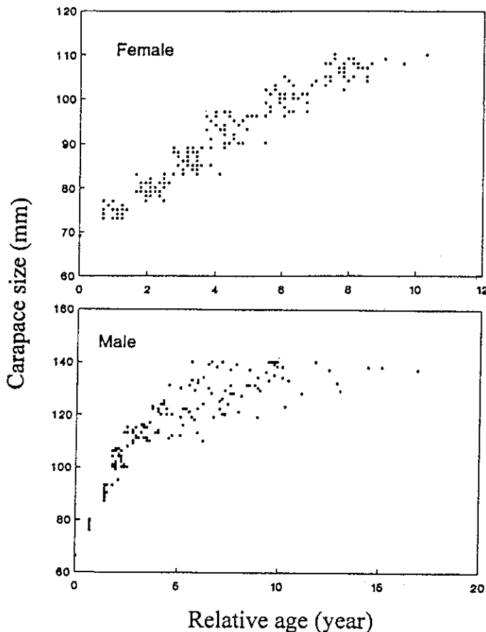
Fig. 6. Scatterplot of size at relative age generated from 100 simulation runs using the probabilistic stepwise growth simulation approach.
