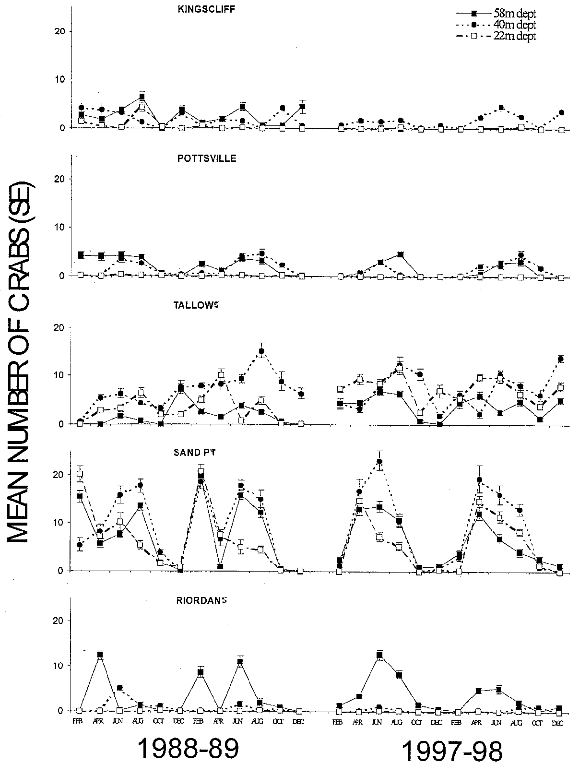
Figure 10. Fluctuations in the mean catch rate ( \pm SE) of undersize spanner crabs during both repeats of the survey at each location and depth ( n = 15 ).
