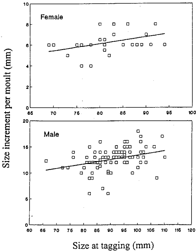
Fig. 4. Frequency of size increment per moult for spanner crabs of different size classes.
