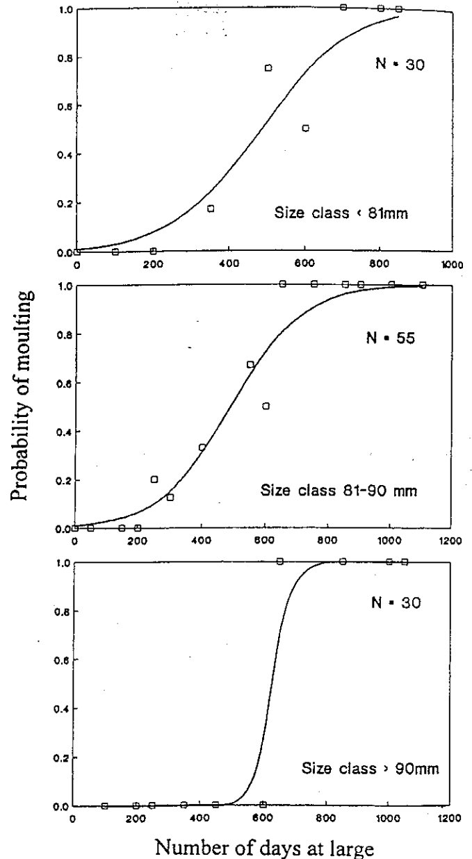
Fig. 2. Probability of moulting for female spanner crabs of different size classes in relation to the number of days at large: \square , observed value; curve, predicted value.
