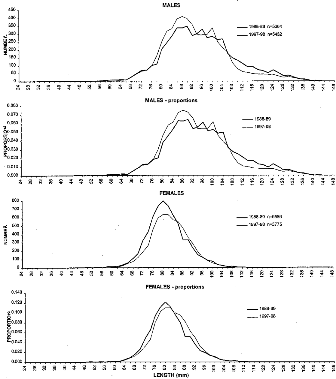
Figure 5. Size-frequencies of male and female spanner crabs sampled during both repeats of the survey.
