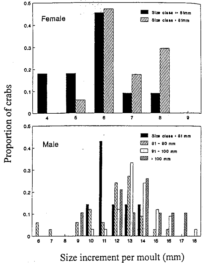
Fig. 5. Relationship between size increment per moult and pre-moult size.
