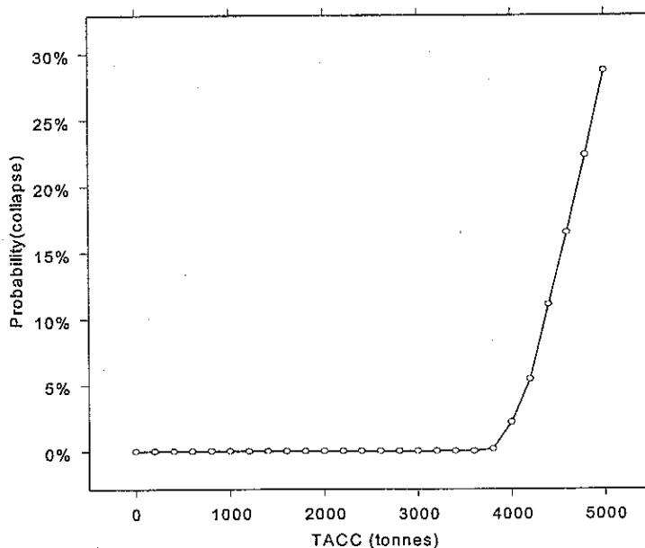
Figure 19. Plot illustrating the probability of collapse in the exploitable biomass as a function of TACC for the combined NSW and Queensland fishery. Note that the spawning biomass is essentially not vulnerable in this fishery and there is no suggestion that the spawning stock will collapse. Risks to the exploitable stock become evident at a harvest rate of around 3 800 tonnes/year. This model will generate less reliable results for the entire fishery than those suggested for the NSW fishery.
