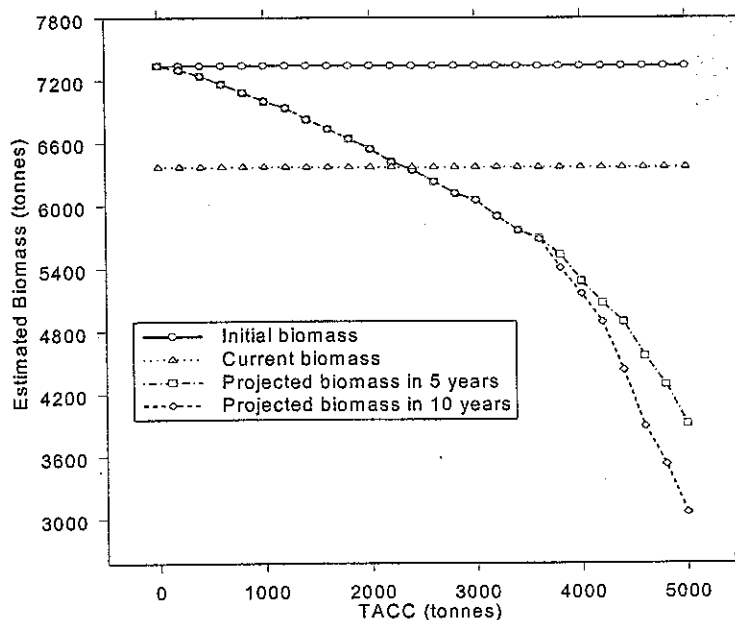
Figure 18. Plot of the median values of the biomass estimates for various total allowable commercial catches (TACC) for the combined NSW and Queensland fishery. The initial and current biomass estimates are independent of TACC (as expected). This model will generate less reliable results for the entire fishery than those suggested for the NSW fishery.
