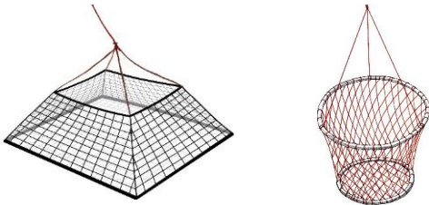
Figure 10. Open pyramid lift net and hoop net
