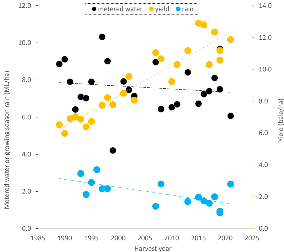
Figure 2. Cotton yield, rainfall and irrigation water trends: The trend of rising cotton yields since the 1990s (represented by the yellow dots) has occurred while total growing season rainfall (blue dots) and irrigation water use on farm (black dots) has been trending downwards. Data prior to 2019 are redrawn from previous benchmarking (Tennakoon and Milroy 2003; Williams and Montgomery 2008; Montgomery and Bray 2010; Roth et al. 2013; Montgomery et al. 2014).
