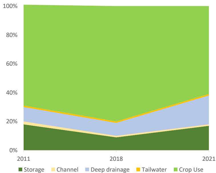
Figure 4. The partitioning of irrigation water into crop use and various on farm losses from 2011, 2018 and in 2021: The proportion of seepage and storage losses doubled from 2018 to 2021 due to a very wet season.
