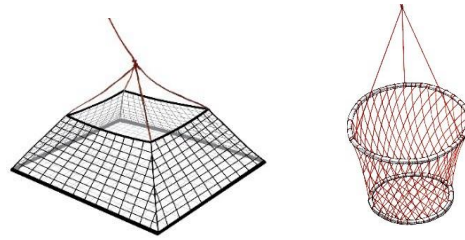
Figure 9. Open pyramid lift net and hoop net
