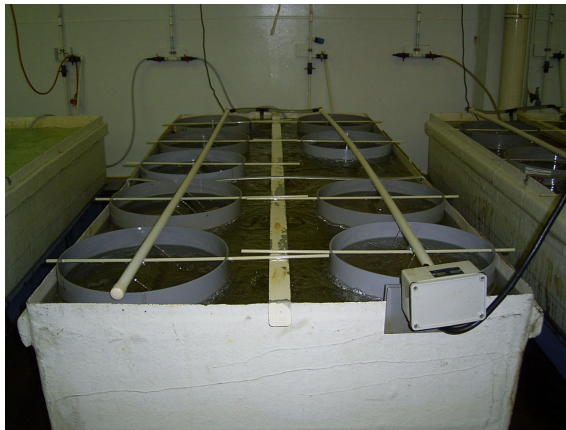
Setting tank holding 10 settlement screens. Settlement screen downwelling
