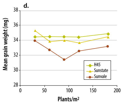
Figure 1–8: Effect of plant population in three wheat varieties on a) grain yield, b) head density, c) grain number per head and d) mean grain weight, Dubbo 2003.
