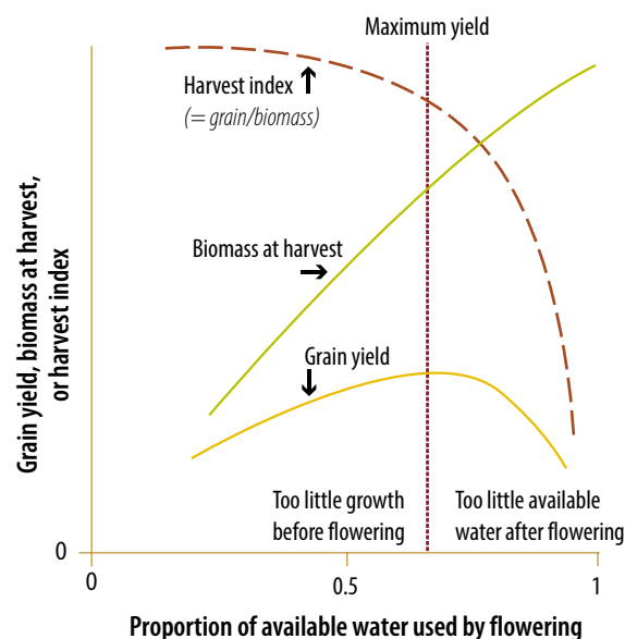
Figure 4–9: The proportion of available water supply used for flowering in dryland crops has a large influence on the yield of the crop, depending on the amount of dry matter at harvest.
