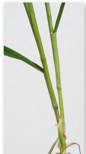
Figure 3–6: Cross-section and photo of the stem, showing the node and the swollen leaf base that can be felt as a hard lump. Source: Illustration, E Kirkby & M Appleyard, 1984; photo, L Turton.
