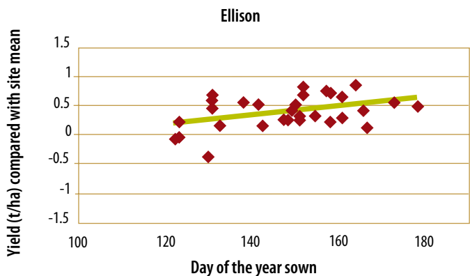
Figure 2–12: Yield responses of different varieties to sowing day. Variety response to sowing time is measured by grain yield (t/ha) relative to the site mean. The site mean is set to zero and graphed against the day of the year sown. 15 May = year day 135.
