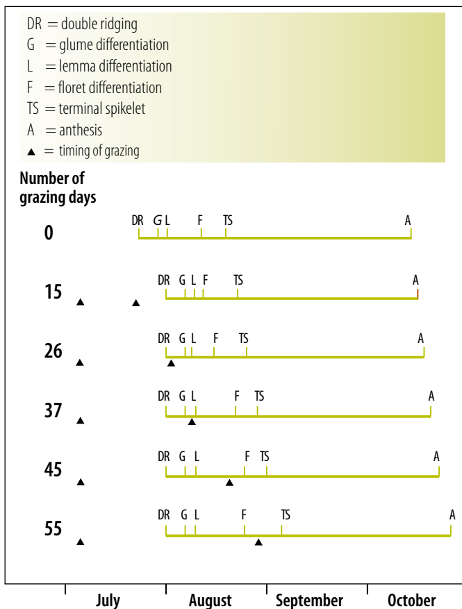
Figure 3-17: Grazing and development of wheat, Cookardina 2004 Source: Based on J Virgona, F Gummer & J Angus, 2006.
