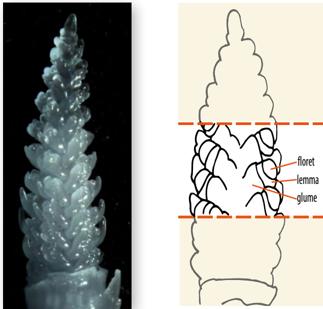
Figure 3-3: The initiation of the spikelet and florets. The most advanced spikelets are in the mid part of the apex. Source: photo, CSIRO; illustration, E Kirby & M Appleyard, 1984.
