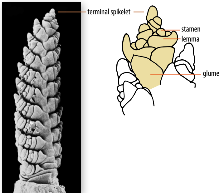
Figure 3-4: The structure of the head at the terminal spikelet stage with illustration showing the terminal spikelet. The apex is about 4 mm long and is just above the soil surface. Source: photo, CSIRO; illustration, E Kirby & M Appleyard, 1984.
