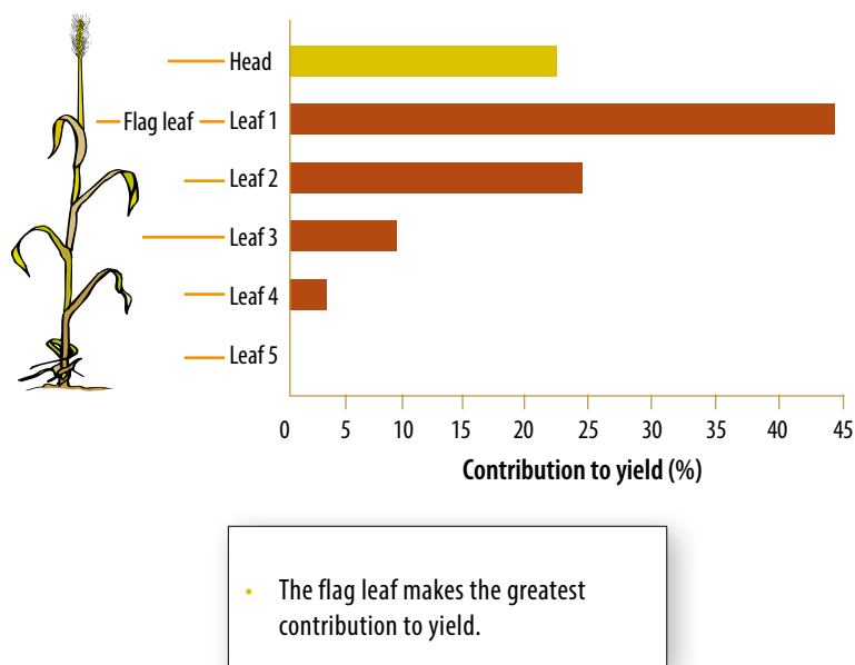
Figure 4-2: Photosynthetic contribution of plant parts. Source: Based on N Fettell, 2006, NSW Department of Primary Industries technical update.
