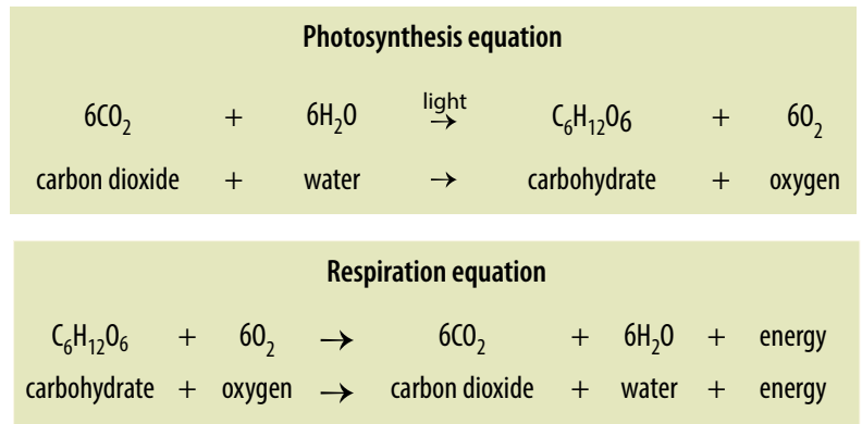
Figure 2–5: Equation for photosynthesis and respiration.
