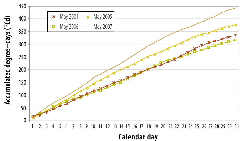
Figure 2–10: Variation in the thermal time across 4 years for the month of May at Cowra. Source: J Edwards, District Agronomist, Cowra 2007.
