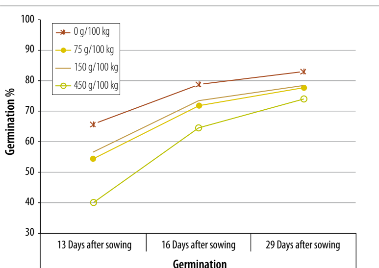
Figure 1-5: Impact of fungicide on the rate of germination. Source: Based on P Cornish, 1986.
