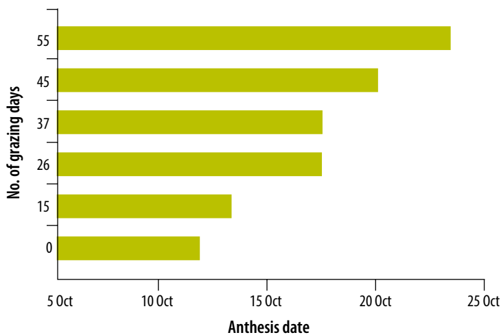
Figure 3-18: Impact of grazing on development at Cookardina 2004. Source: Based on J Virgona, F Gummer & J Angus, 2006.
