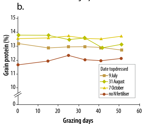
Figure 4–8: (a) Yield and (b) grain protein in crops grazed for different durations and managed with different nitrogen (N) fertiliser strategies. Topdressed with 60 kg/ha of N fertiliser on the dates specified. The bars indicate least significant difference. Source: Based on J Virgona et al., 2006.
