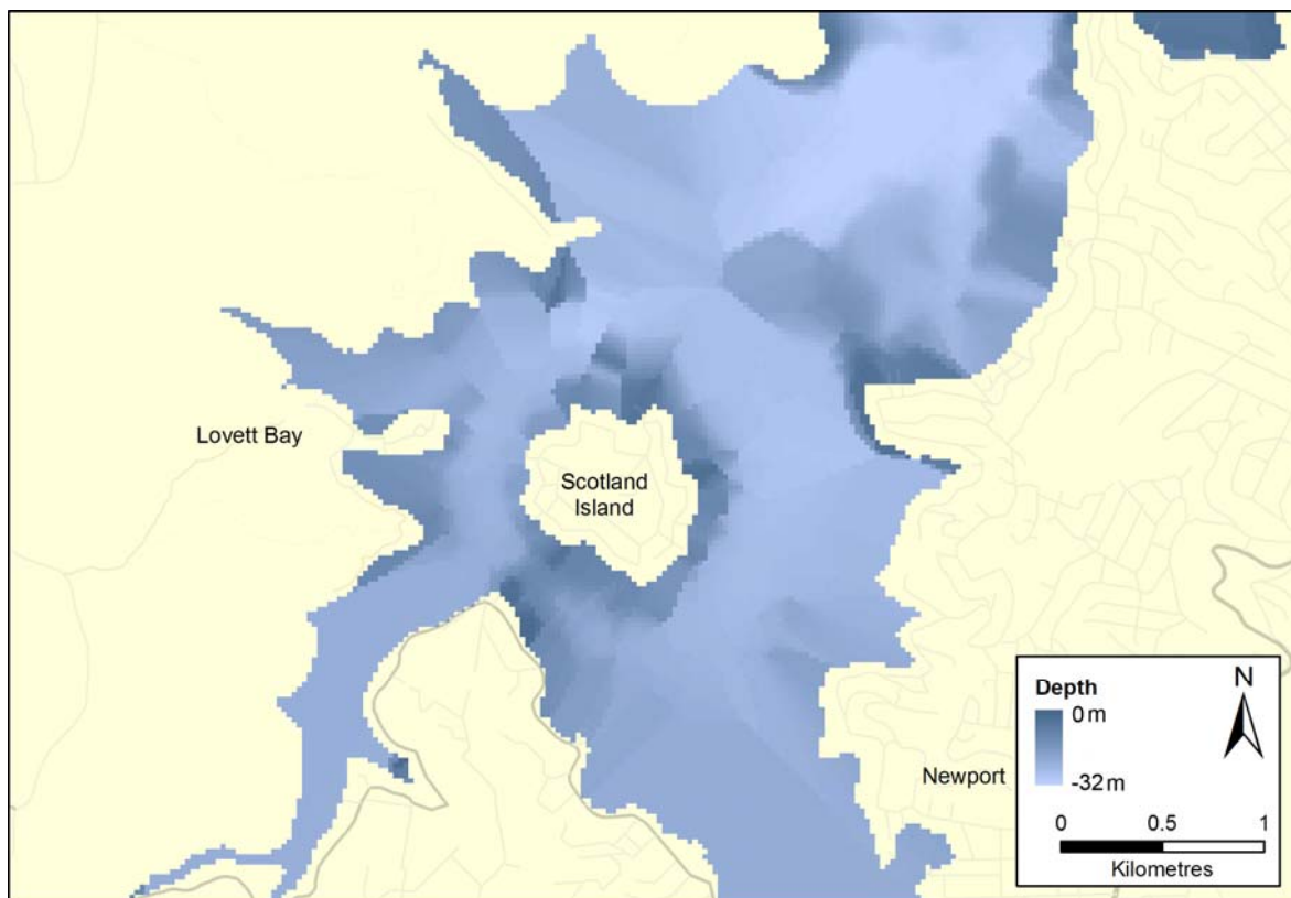
Figure A.1. Detailed gridded bathymetry of Pittwater. This dataset is a composite of several different datasets that vary in spatial extent and resolution.
