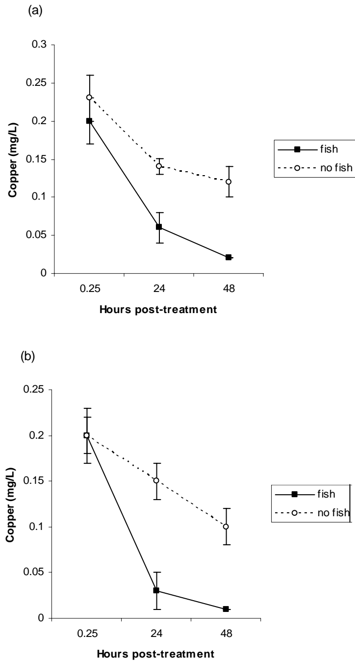
Figure 6.4.7. Depletion of copper in aerated, 0.1-ha earthen ponds with and without fish at (a) trial 1 – mean water temperature 14.8°C (13.3° – 16.6°C) and (b) trial 2 – 20.9°C (19.5° – 22.4°C). Data are means \pm SD of three replicate ponds.
